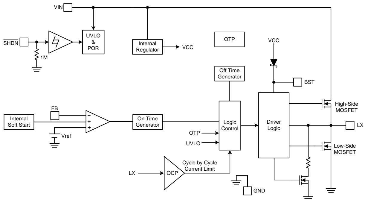
Figure 3. Block Diagram of FR9205F
